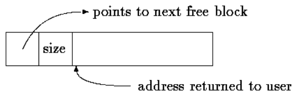
A block returned by malloc
