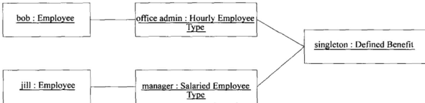
图 16-20 每个 Employee Type 被指定一个 Retirement Plan
