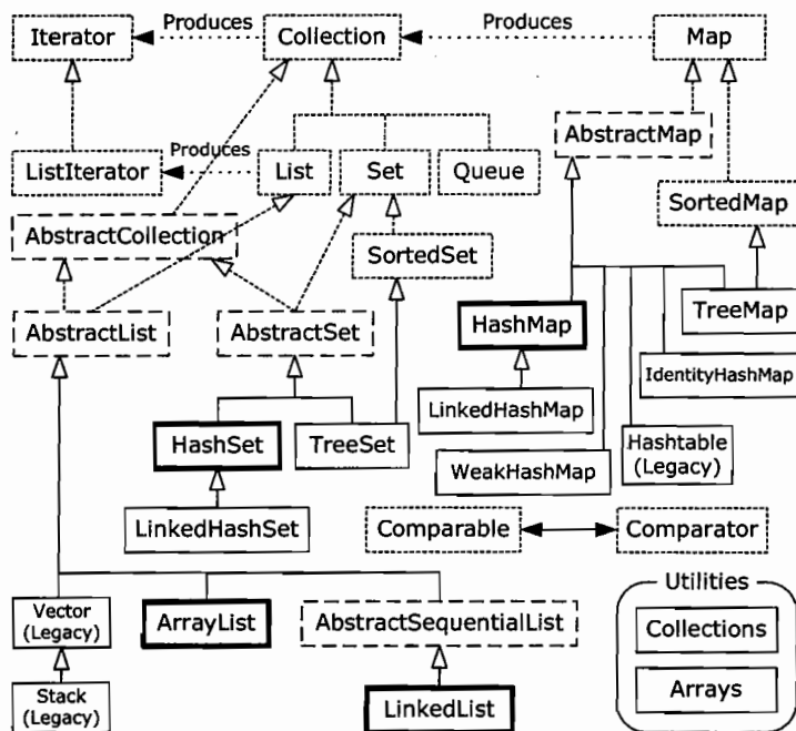
Full Container Taxonomy
