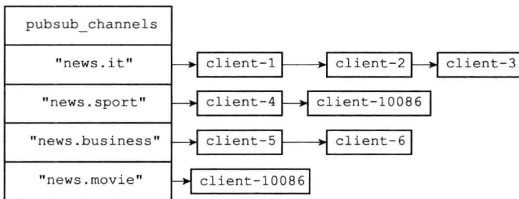
图 18-19 pubsub_channels 字典
