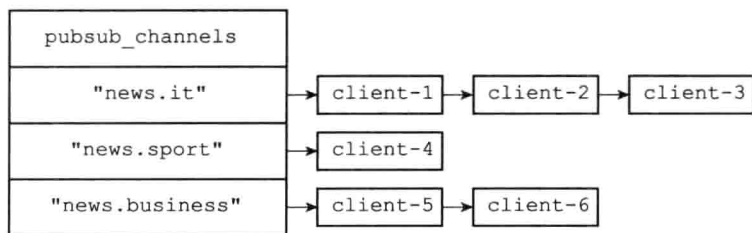
图 18-16 pubsub_channels 字典
